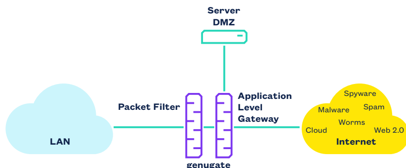
The two-tier firewall genugate combines two different firewall systems – an application level gateway and a packet filter
